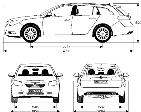
Sports Tourer alle afmetingen in mm
